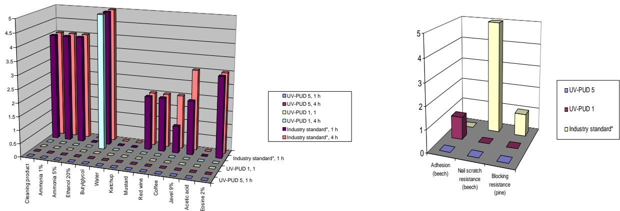
Chemical resistance DIN 68 864 (0 = very good, 5 = bad)
