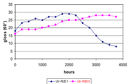
Comparative ageing on neutral substrate
